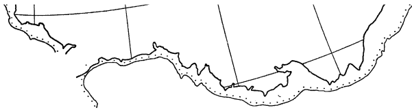
at the 500 fm. contour, transverse Mercator projection.
