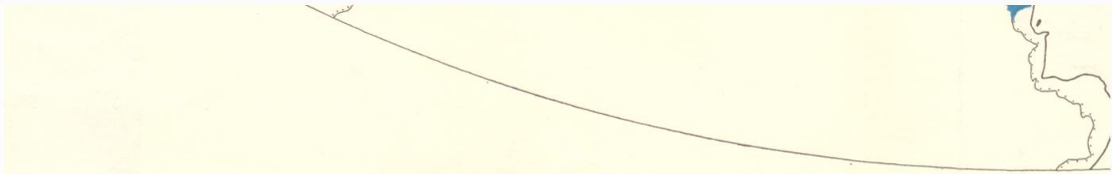
FIGURE 7. The fit of North America, Greenland and Europe at the 500 fm. contour
