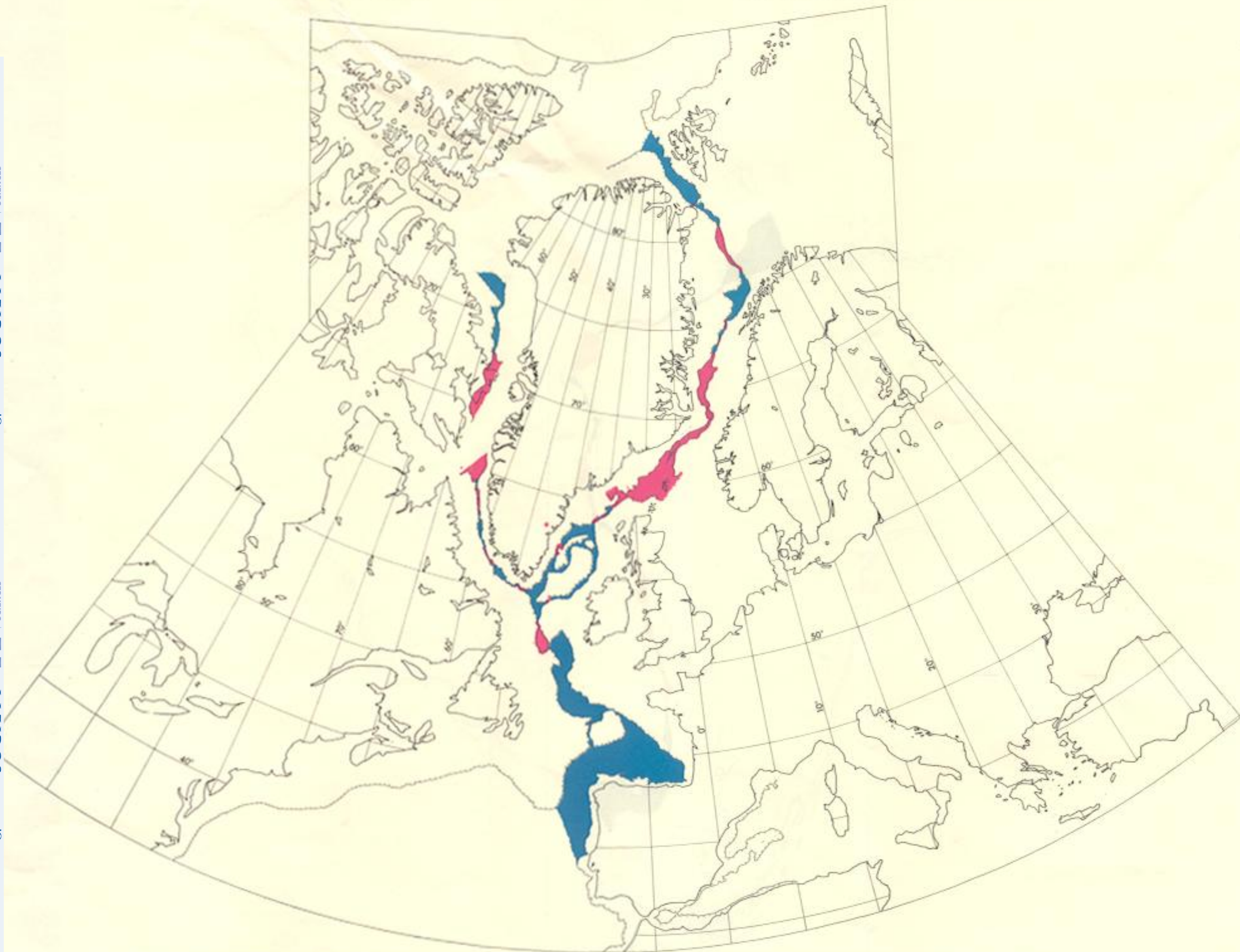
FIGURE 7. The fit of North America, Greenland and Europe at the 500 fm. contour (fits 1 and 2 of table 2), conical projection. Overlaps in red, gaps in blue.
