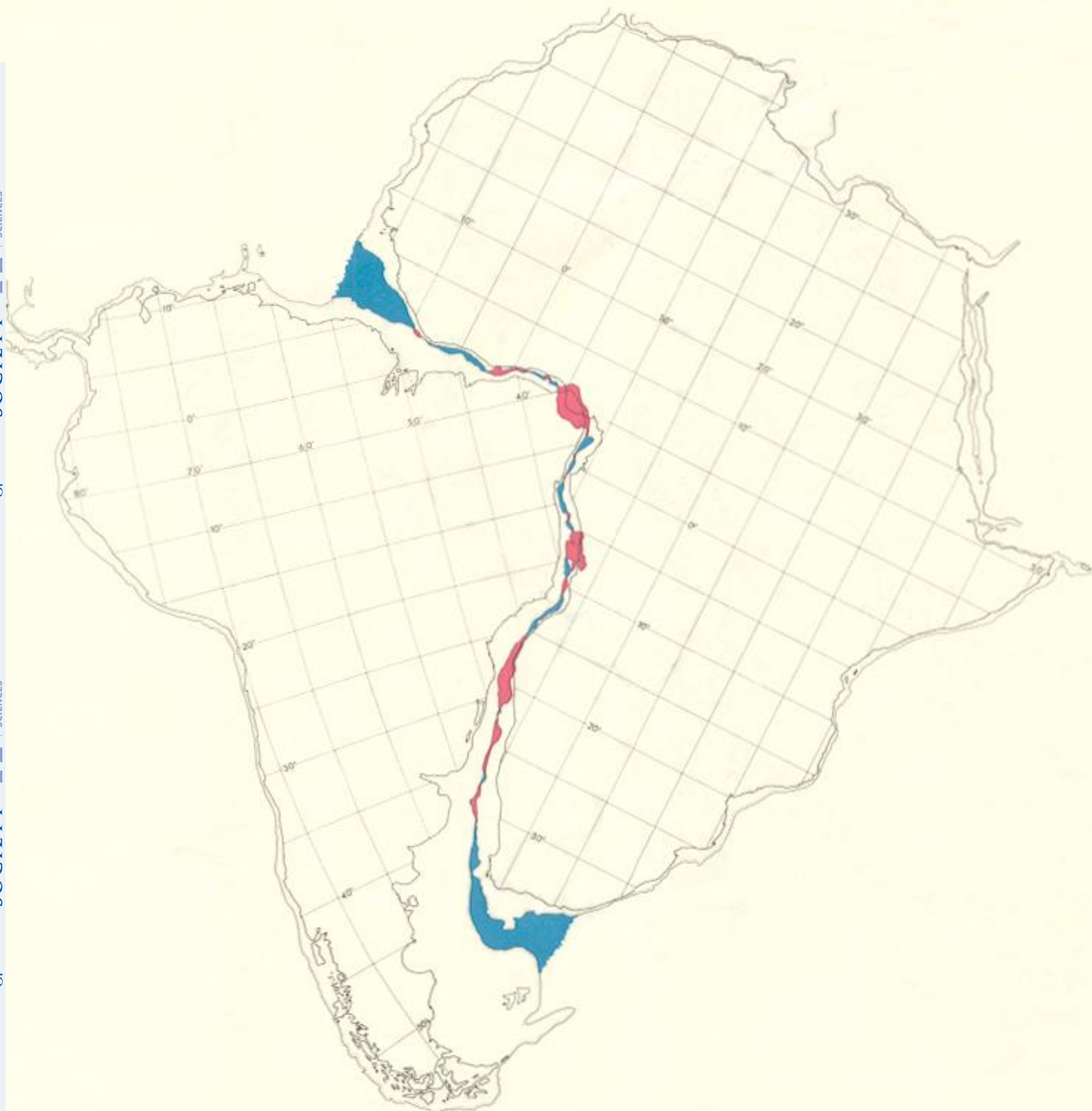
FIGURE 5. The fit of Africa and South America at the 500 fm. contour (fit 9 of table 1), Mercator's projection. Overlaps in red, gaps in blue.
